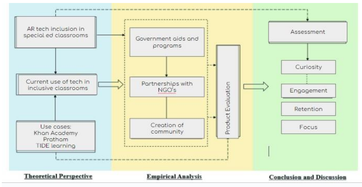
Fig 1.5 Research Framework
